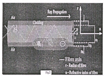
Fig: 2) Multimode step index optical fiber
